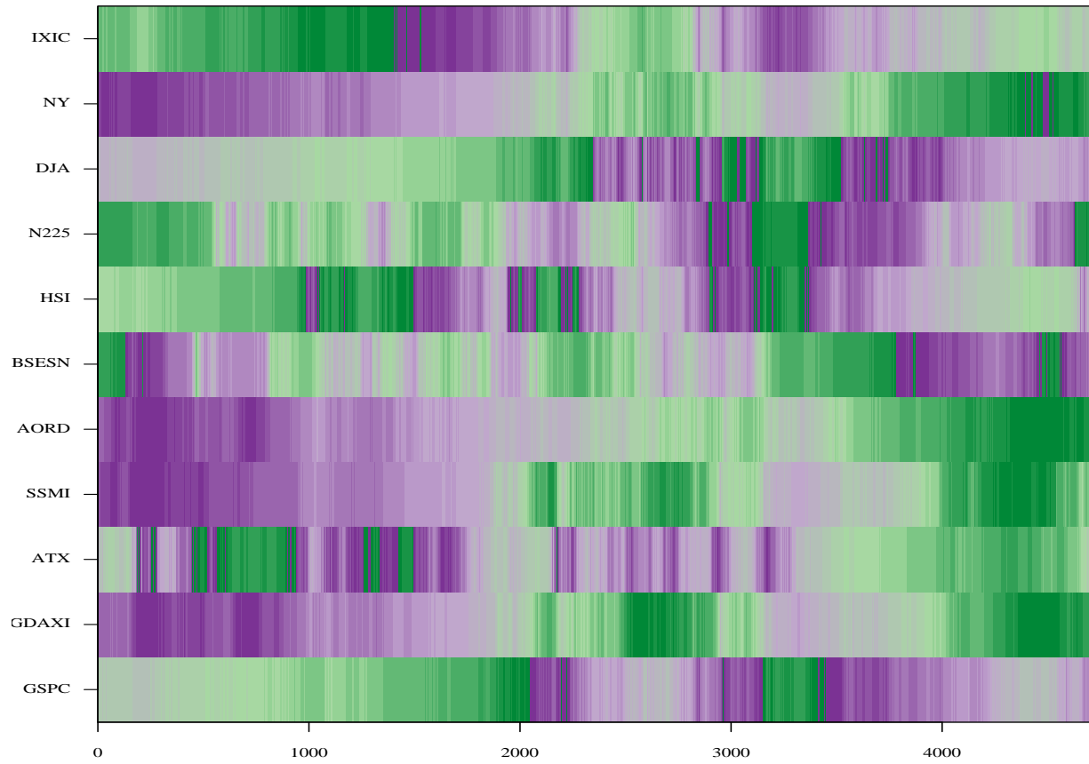
FIG. 7: Histogram-based (i.e., non-entropic) heat map between the 11 stock indices listed in Appendix A.
