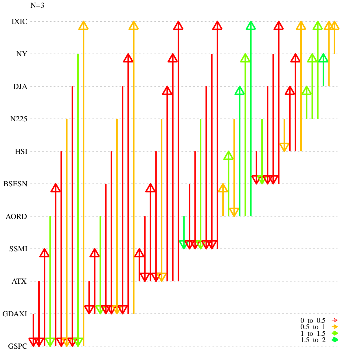
FIG. 9: Net flow F_{Y \leftrightarrow X} of effective Shannon transfer entropies between the 11 stock indices listed in Appendix A. Alphabet size N = 3 .
