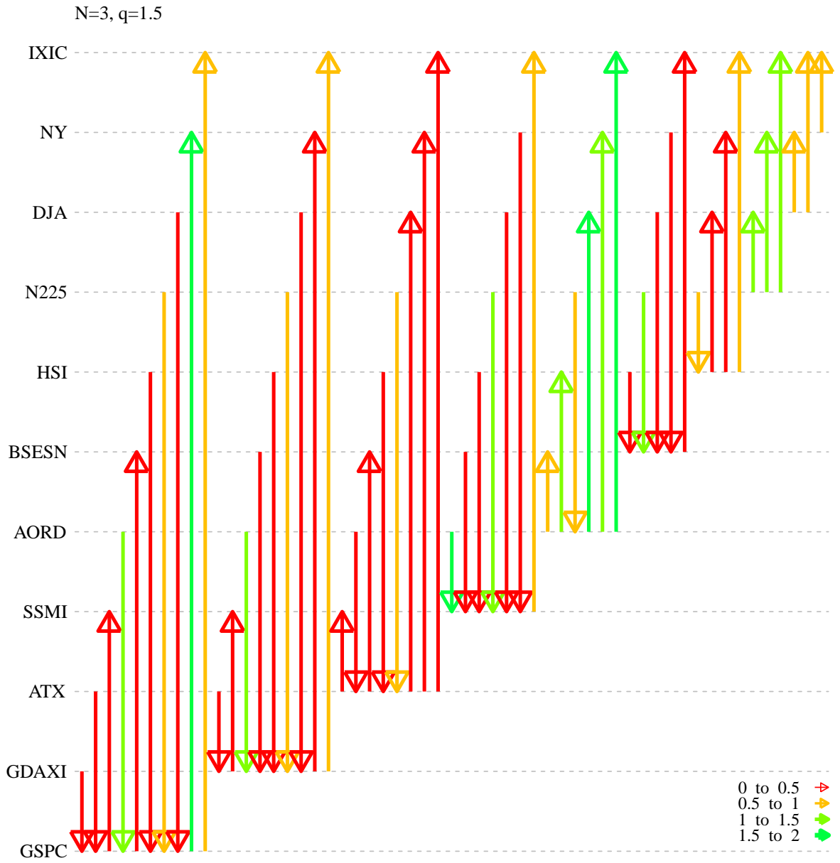
FIG. 11: Net flow F_{Y \leftrightarrow X} of the effective Rényi transfer entropies listed in Appendix A; q = 1.5 . Alphabet size N = 3 .
