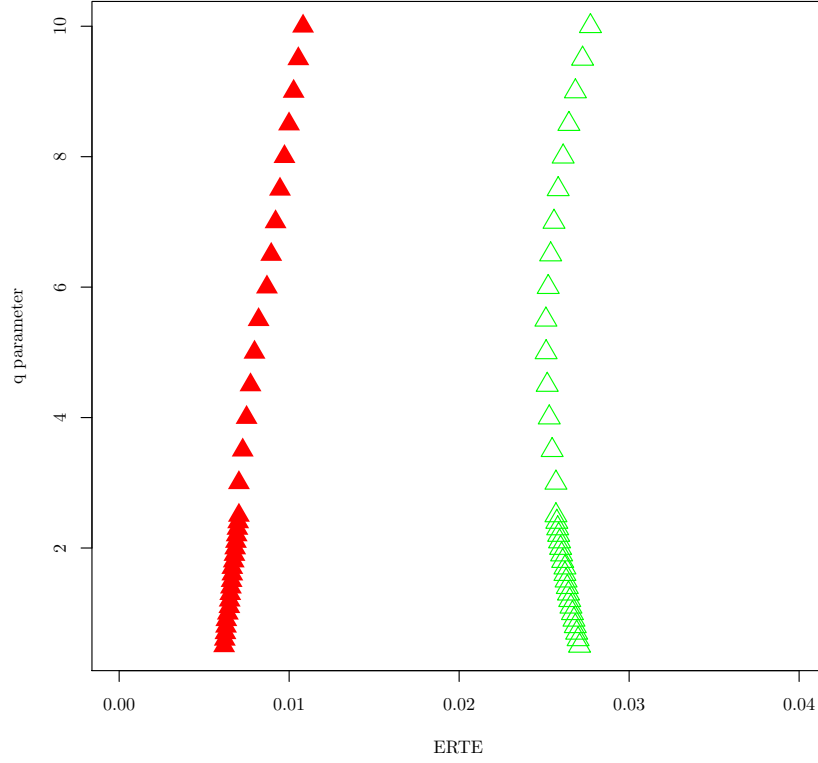
FIG. 16: The ERTE as a function of q . The alphabet size is set to N = 3 . DAX and SP&500 minute prices are employed. The red curve corresponds to T_{q;SP\&500 \rightarrow DAX}^{(R, \text{eff})}(m, m) while the green curve denotes T_{q;DAX \rightarrow SP\&500}^{(R, \text{eff})}(m, m) .
