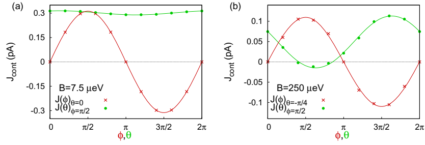
Figure 8. Numerical results for the continuum contribution to the Josephson current as a function of \phi (red crosses) and \theta (green dots). The solid lines are fits to the \phi -derivative of equation (4), \partial_\phi E_{\text{cont}}(\phi, \theta) . All parameters are the same as in figure 7. The fixed angle is chosen such that the current is maximized. In this way, the oscillation amplitudes can be used to obtain J_\phi and J_\theta plotted in figure 7. The \phi dependence is simply J(\phi) = J_\phi \sin(\phi) . In contrast J(\theta) has a large offset and only a weak \theta dependence for B \sim \Delta (panel (a)). This corresponds to \alpha \sim 1 . For B \gg \Delta (panel (b)), the amplitude of J_\theta approaches that of J_\phi and \alpha decreases.
