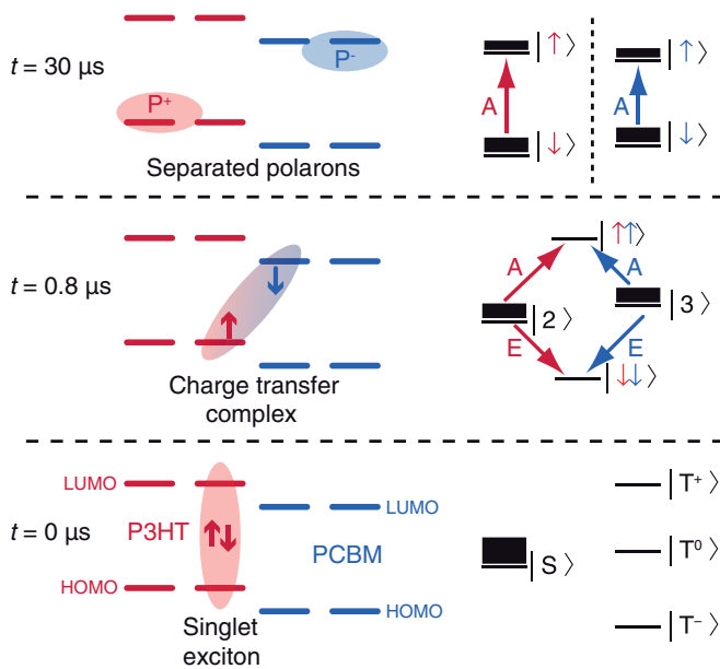
FIG. 2. (Color online) Schematic energy diagram of the HOMO and LUMO levels of P3HT and PCBM (left) and corresponding spin-pair eigenstates of a charge transfer complex consisting of two S = 1/2 particles (right) along with the EPR-active transitions (as indicated by the arrows), which give rise to absorptive ( A ) and emissive ( E ) signals in the trEPR spectrum. From bottom to top, a singlet exciton ( |S\rangle ) is created upon photoexcitation of the P3HT. Subsequently, this is converted into a CTC, with the mixed states |2\rangle and |3\rangle being populated and the pure triplet states |\uparrow\uparrow\rangle and |\downarrow\downarrow\rangle being unpopulated (as indicated by the according horizontal bars). Finally, the CTC dissociates into two separated polarons ( P^+ and P^- ) exhibiting thermalized spin populations.
