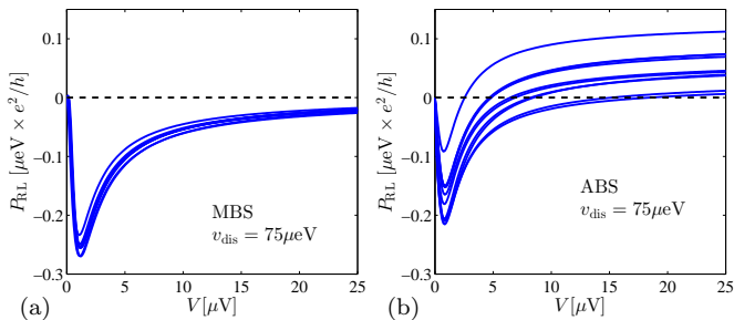
FIG. 3: Current cross correlation P_{\text{RL}} vs. bias voltage V at \mu = 0 and T = 0 for different realization of short-range Gaussian disorder. (a) B = 520\text{mT} > B_c , the system is in the topological phase with a zero-energy Majorana bound state (MBS) at each end of the wire. The universal behavior of P_{\text{RL}}(V) , (being negative and approaching zero at high voltage) is not affected by the presence of disorder. (b) For each realization of disorder the magnetic field is tuned to have an Andreev bound state (ABS) with zero energy at the end of the wire, while keeping the system in the topologically trivial phase, B = 170 - 200\text{mT} < B_c (see the text for more details). The behavior of P_{\text{RL}}(V) varies significantly for different realizations of disorder. In all cases P_{\text{RL}} > 0 for large V in contrast to the topological case where it goes to zero.
