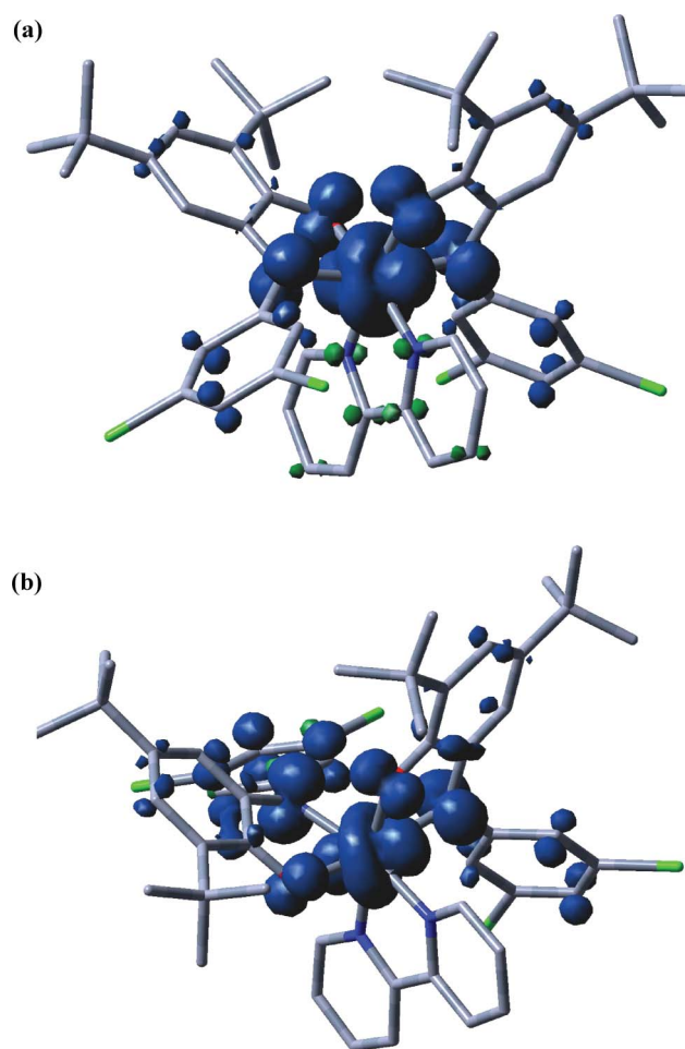
Fig. 11 DFT calculated spin density plots of (a) 2a - and (b) 2b - .
