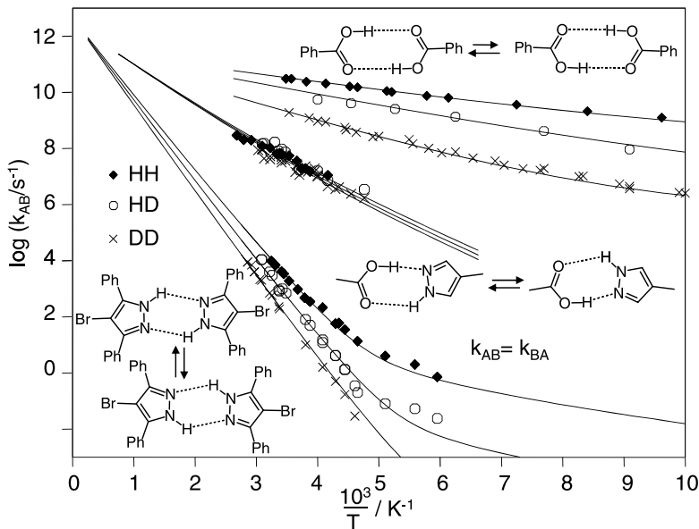
Fig. 11. Comparison of the Arrhenius diagrams of the double proton and deuteron transfers in benzoic acid dimers [1,15], 2,4-diphenyl-3-bromopyrazole dimers [31] and crystalline PCA.
