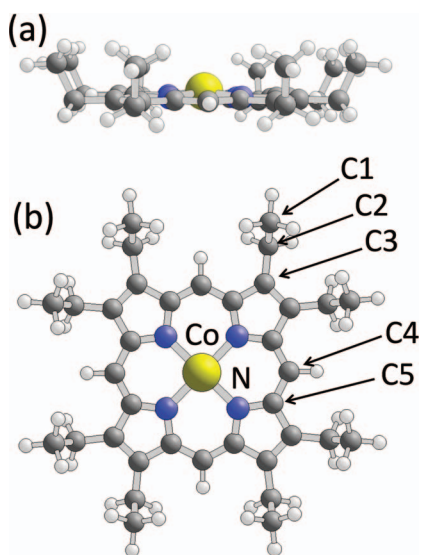
FIG. 1. Geometric structure of the free Co-OEP molecule for (a) a side view and (b) a top view. Atoms are shown by balls of different radii and labeled accordingly.
