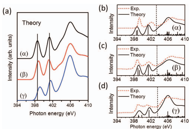
FIG. 7. (a) Theoretical N 1s core excitation spectra for (\alpha) the free Co-OEP molecule, (\beta) the \text{Ni}_4\text{O}-(\text{Co-OEP}) cluster, and (\gamma) the \text{Ni}_4-(\text{Co-OEP}) cluster, see text and Figs. 1 and 2. The vertical lines indicate positions of the two peaks in the free Co-OEP spectrum. (b)–(d) Comparison of the theoretical polarization-averaged N K-edge NEXAFS data with corresponding experimental polarization-averaged N K-edge NEXAFS data, see text. The vertical dotted lines indicate positions of the theoretical ionization threshold in each spectrum.
