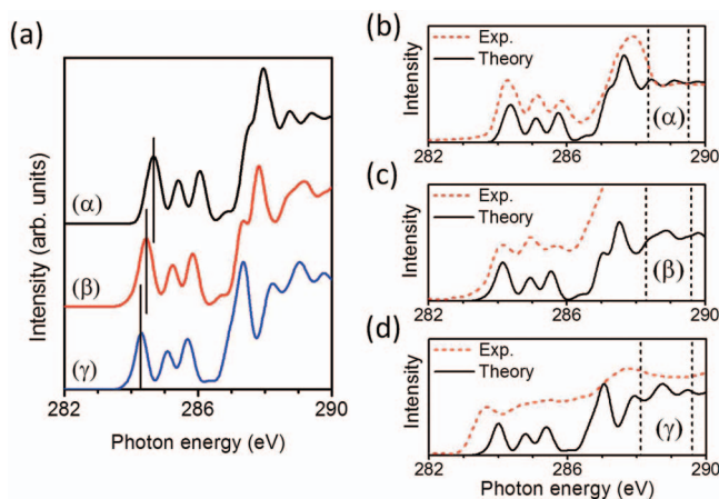
FIG. 5. (a) Theoretical polarization-averaged C 1s core excitation spectra for ( \alpha ) the free Co-OEP molecule, ( \beta ) the \text{Ni}_4\text{O} -(Co-OEP) cluster, and ( \gamma ) the \text{Ni}_4 -(Co-OEP) cluster, see text and Figs. 1 and 2. The vertical lines indicate positions of the energetically lowest peak in each spectrum. (b)–(d) Comparison of the theoretical spectra ( \alpha ), ( \beta ), ( \gamma ) with corresponding experimental polarization-averaged C K-edge NEXAFS data, see text. The vertical dotted lines indicate positions of the theoretical ionization threshold in each spectrum.
