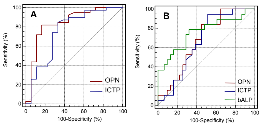
Figure 14 ROC curves of OPN, ICTP, and bALP to differentiate RCC patients with different tumor stages and grades. A. Tumor stages: I versus II-IV. B. Tumor grades: G1-2 versus G3.
