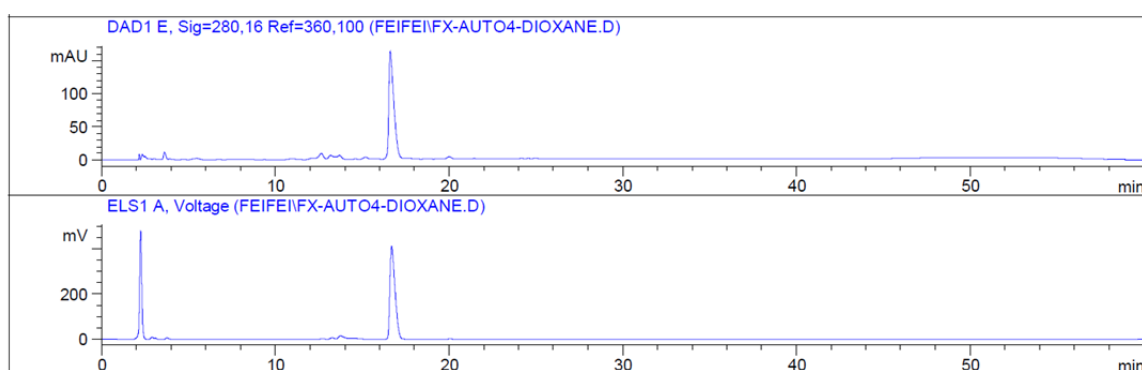
Figure 4.3: Analytical HPLC of the crude disaccharide 99 after UV-cleavage. Column: YMC-Diol-300-NP 5\mu\text{m} ( 150 \times 4.60 mm); mobile phase: ethyl acetate and hexanes.
