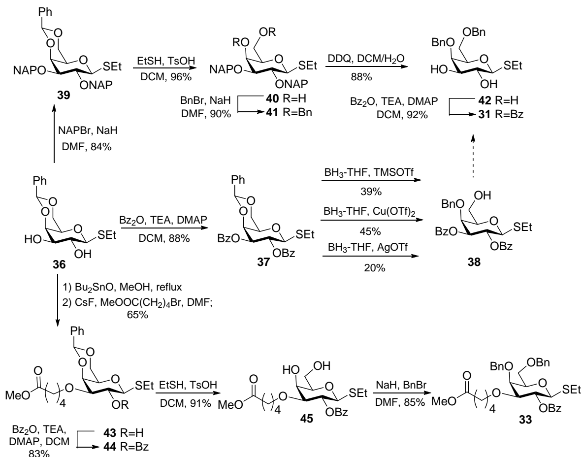
Scheme 2.2: Synthesis of building blocks 31 and 33 .
