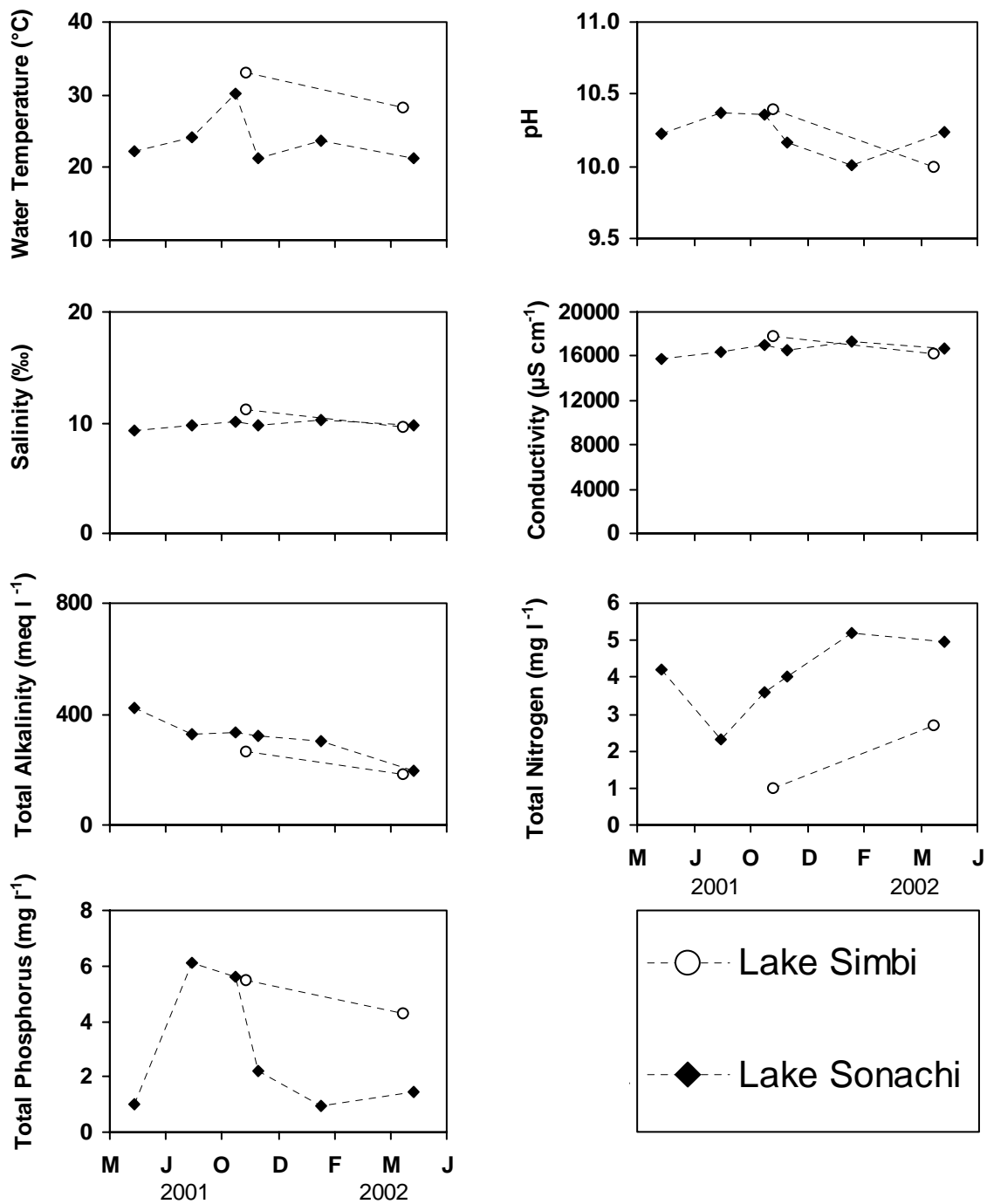
Fig. 1: Physico-chemical conditions in Lake Sonachi and Lake Simbi from June 2001 to June 2002.
