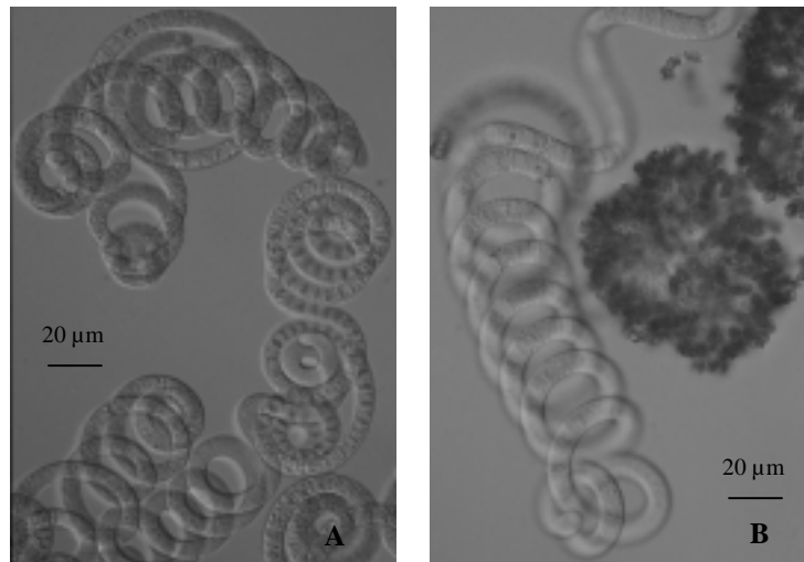
Fig. 2. A) Arthrospira fusiformis from Lake Sonachi;
