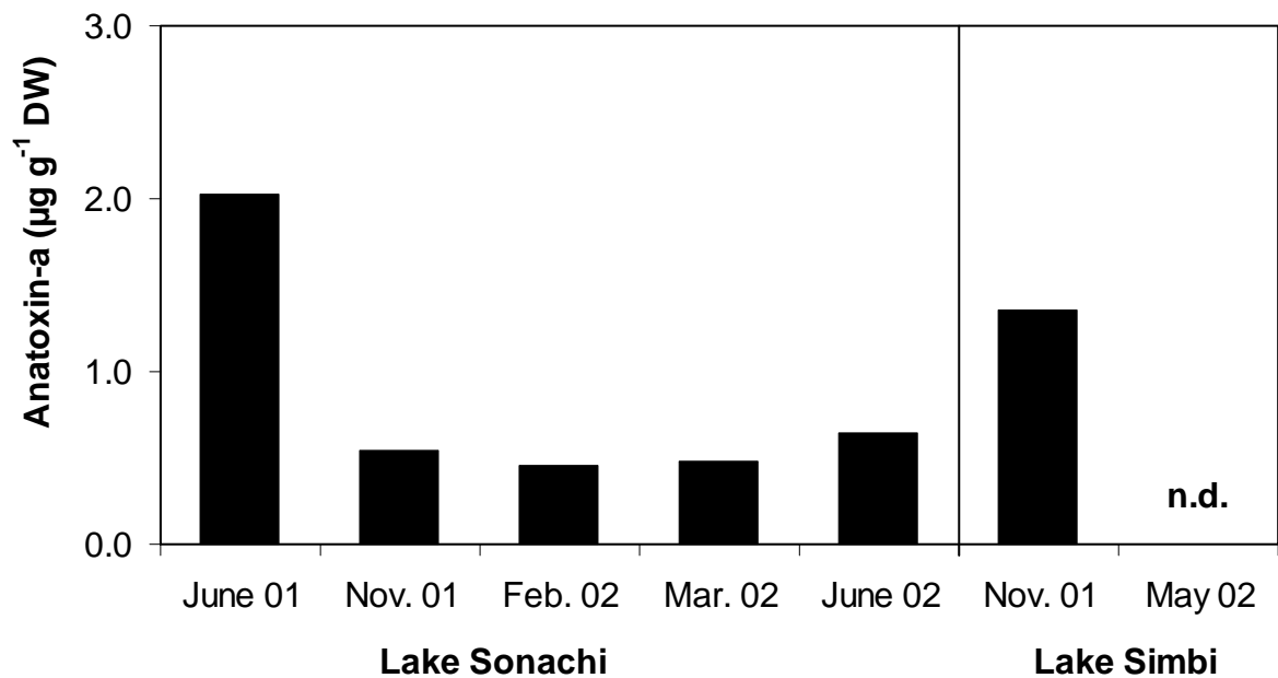
Fig. 5: Anatoxin-a in Lake Sonachi and Lake Simbi in the samples from June 2001 to June 2002. n.d. = not detected.
