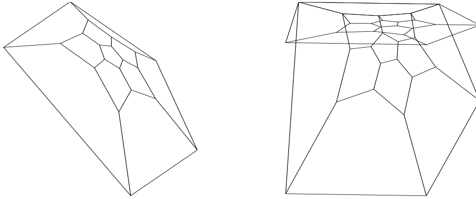
Figure 3.4: Two pictures of the dodecahedron embedded with our algorithm with scaled z -axis. The right picture includes also the equilibrium stressed plane embedding.
