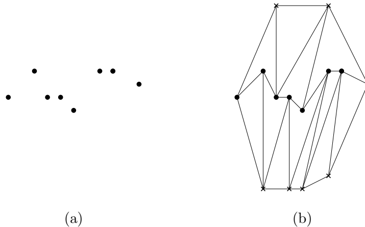
Figure 7.1: A point set (a) and its degree 4 pseudo-triangulation with O(n) Steiner points drawn as crosses (b).
