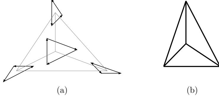
Figure 2.2: Constructing the Maxwell reciprocal.
