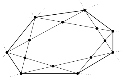
Figure 5.13: The planarization technique for graphs with equilibrium stress. For showing that the graph has a planar embedding the diagonals of the triangulations can be drawn in the outer face.
