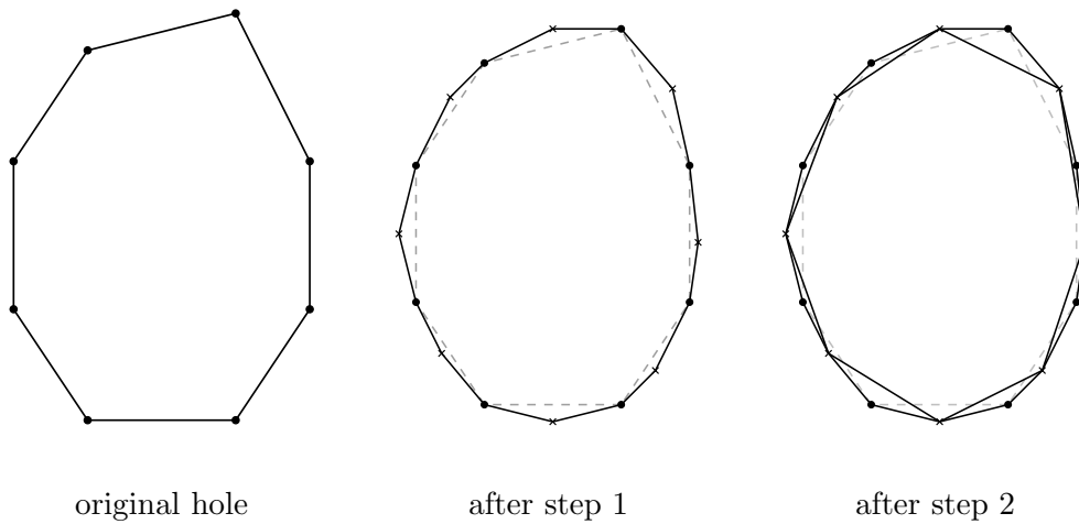
Figure 6.21: Step 1 and 2 for filling the holes. The crosses mark newly added vertices. Original hole edges are drawn dashed.
