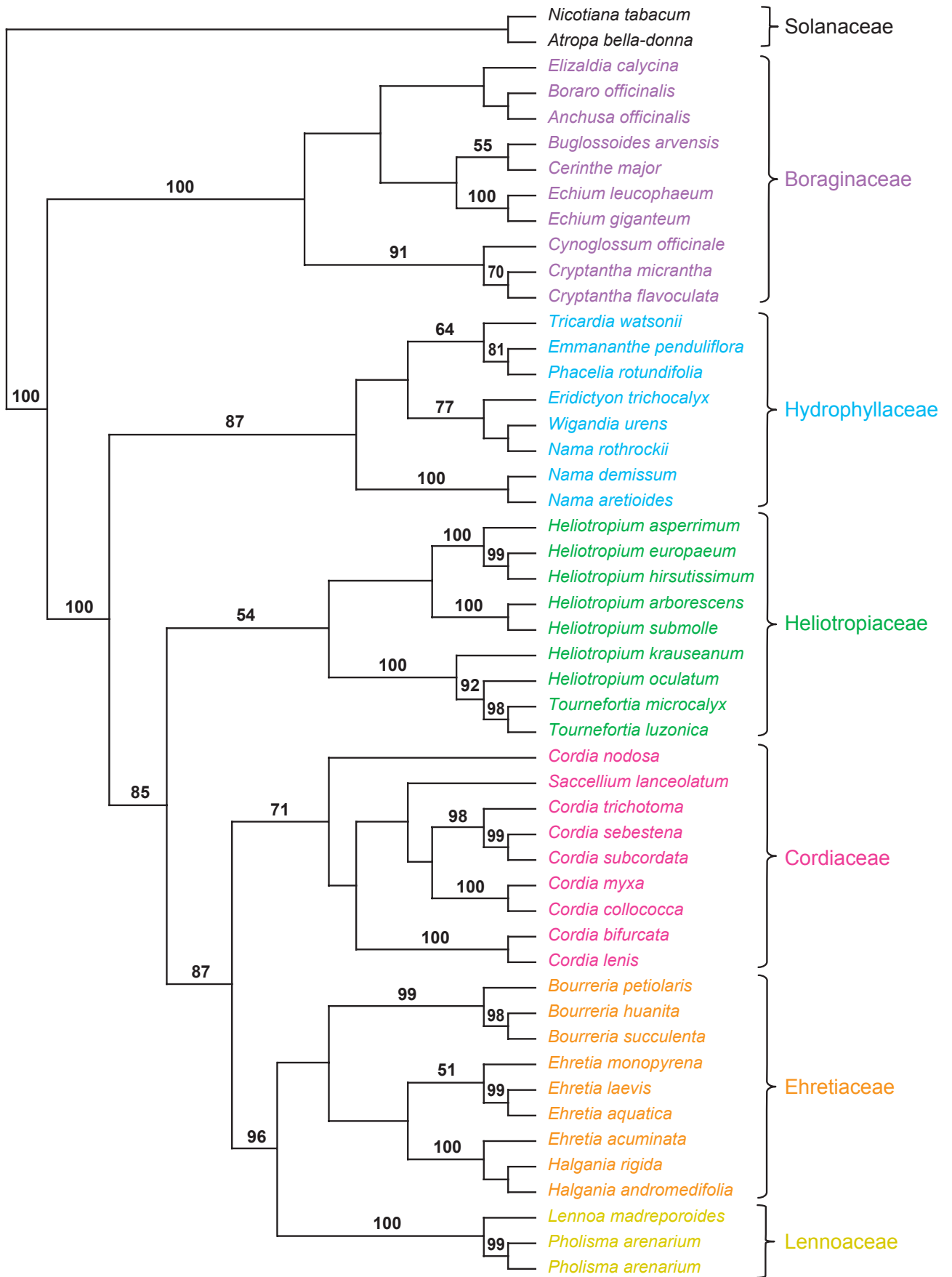
Fig. 3-10. One of five most parsimonious trees of Boraginales (L = 383, CI = 0.50, RI = 0.65). Important taxa are indicated. The numbers above branches are bootstrap support values to the clusters to the right of them (values under 50% not shown).
