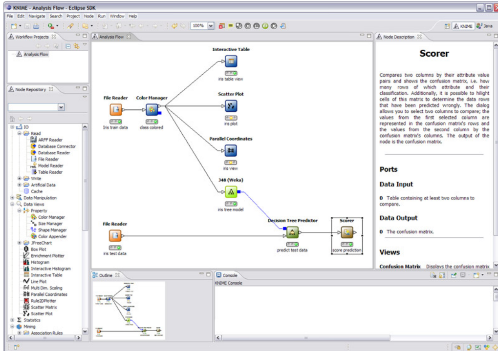
ABBILDUNG 4.3: Workflow-Engine KNIME
