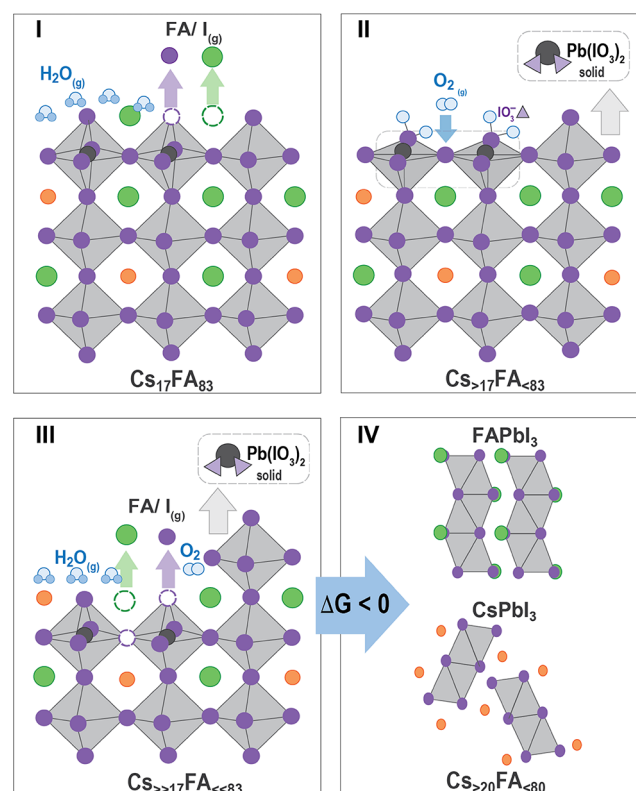
Figure 4. Proposed surface and bulk mechanism for CsFA perovskites exposed to H 2 O/air. (I) H 2 O is adsorbed on the CsFA surface, promoting the loss of FAI (g). Surface vacancies are created, leading to preferential oxygen binding sites, favoring the oxidation of iodide and energetically favorable formation of Pb(IO 3 ) 2 (II), which will create a PbI 2 vacancy (III). Surface vacancies and the loss of FAI will lead to faster phase segregation and phase transformations from mixed-cation perovskite into single-cation nonperovskite phases (IV).
