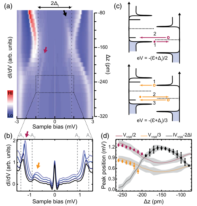
FIG. 4. (a) Closer view of the approach set in Fig. 3(b). (b) Four spectra (offset for clarity) of this set showing two peaks due to the Andreev processes depicted in (c). An electron (hole) is reflected through the junction until its energy matches the YSR state. (d) Extracted positions of the peaks shown in (a) and (b) (rectangles) as well as traces showing the expected positions of a thermal excitation of the YSR state (black trace) and of the processes shown in (c) (yellow and pink) given the position of the YSR state.
