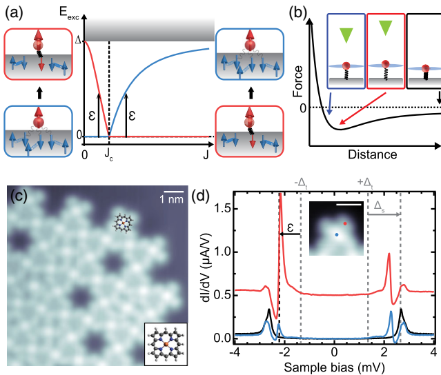
FIG. 1. (a) Schematic dependence of ground and excited states of a magnetic adatom on a superconducting substrate on exchange coupling strength J . At weak coupling, the ground state is a free-spin state, while the excited state has a quasiparticle bound to the adatom. At a critical coupling J_c , the roles of ground and excited states reverse. (b) Sketch of the forces acting between tip and molecule vs tip-molecule distance. At large distances, attractive forces pull the molecule away from the surface. At closer distance, repulsive forces push the molecule back towards the surface. (c) STM topography image of a FeP island ( V = -45 mV, I = 50 pA) with a molecular model (inset). (d) dI/dV spectra acquired with a Pb tip above bare Pb(111) (black), center (blue), and ligand (red, offset for clarity) of a molecule.
