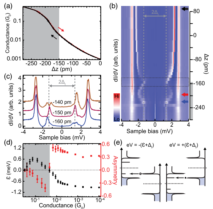
FIG. 2. Tip approach above Fe center of a FeP molecule (for more data, see [32]). (a) Junction conductance (in G_0 = 2e^2/h ) vs tip offset \Delta z . (b) 2D false-color plot of dI/dV spectra recorded at various tip-sample distances, normalized to their conductances at 5 mV. The spectra were acquired after opening the feedback at V = 5 mV, I = 200 pA and subsequently varying the tip height by an offset \Delta z (lock-in modulation V_{\text{rms}} = 15 \mu\text{V} ). (c) Spectra before ( \Delta z = -140 pm, brown trace), at ( \Delta z = -150 pm, claret), and after ( \Delta z = -160 pm, blue) the quantum phase transition (offset for clarity). (d) Extracted YSR energies and intensity asymmetries vs junction conductance. Error bars determined from peak widths and noise level of the spectra. Around G = 0.02 \times G_0 ( \Delta z = -150 pm), the YSR state energy crosses zero and the asymmetry changes sign, indicating the quantum phase transition. (e) Single-electron tunneling processes for YSR resonances at positive and negative bias voltages.
