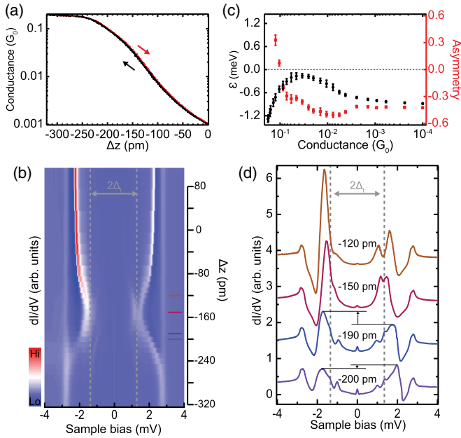
FIG. 3. Tip approach above Fe ligand of FeP molecule [see Fig. 1(b)] (for more data see [32]). (a) Evolution of conductance with tip offset \Delta z . (b) 2D false-color plot of dI/dV spectra recorded at various tip-sample distances, normalized to their conductances at 5 mV. (c) Extracted YSR energies and intensity asymmetries vs junction conductance. (d) Four spectra of this approach set (offset for clarity). The YSR state does not reach zero energy and the asymmetry remains positive during most of the approach [see the brown, claret, and blue spectra in (d)]. The asymmetry reverses only around G = 0.1 \times G_0 , where Andreev reflections become dominant [see blue and purple spectra in (d)].
