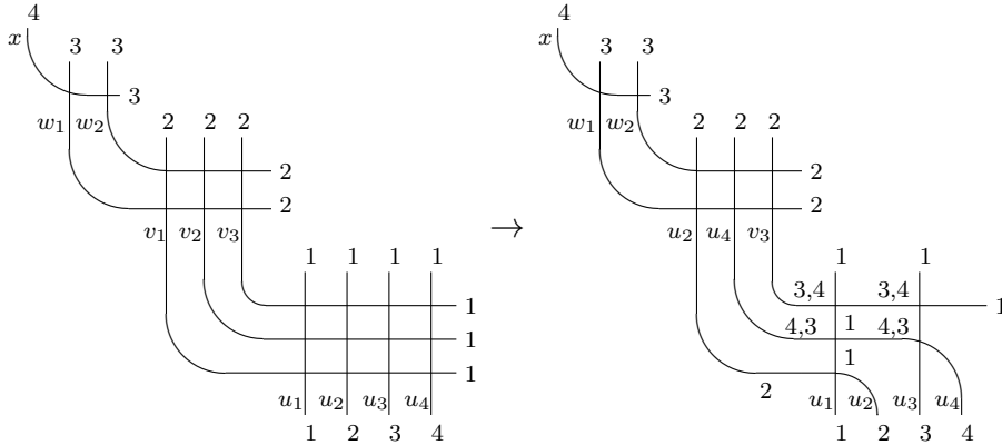
Figure 5: The Bethe state \Psi_{\underline{A}}(\underline{u}, \underline{v}) in (21) for an iso-scalar operator where \underline{A} = (1, 2, 3, 4) and v_1 \rightarrow u_2, v_2 \rightarrow u_4 .
