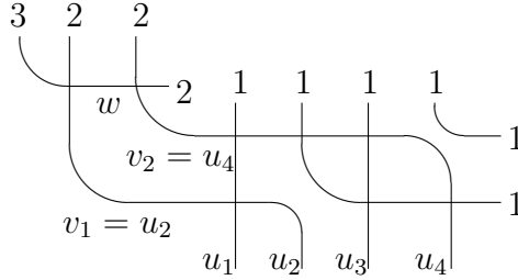
Figure 3: The Bethe state \Psi_{\underline{A}}(\underline{u}, \underline{v}) in (42) for v_1 = u_2, v_2 = u_4 .
