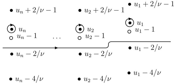
Figure 4: The integration contour \mathcal{C}_{\underline{u},\nu} in (52). The bullets refer to poles of the integrand resulting from \tilde{\phi}(u_i - v_j) and the small open circles refer to poles originating from \tilde{b}(u_i - v_j) and \tilde{c}(u_i - v_j) .
