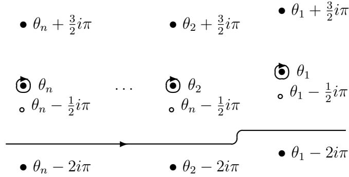
Figure 2: The integration contour for SU(4)
