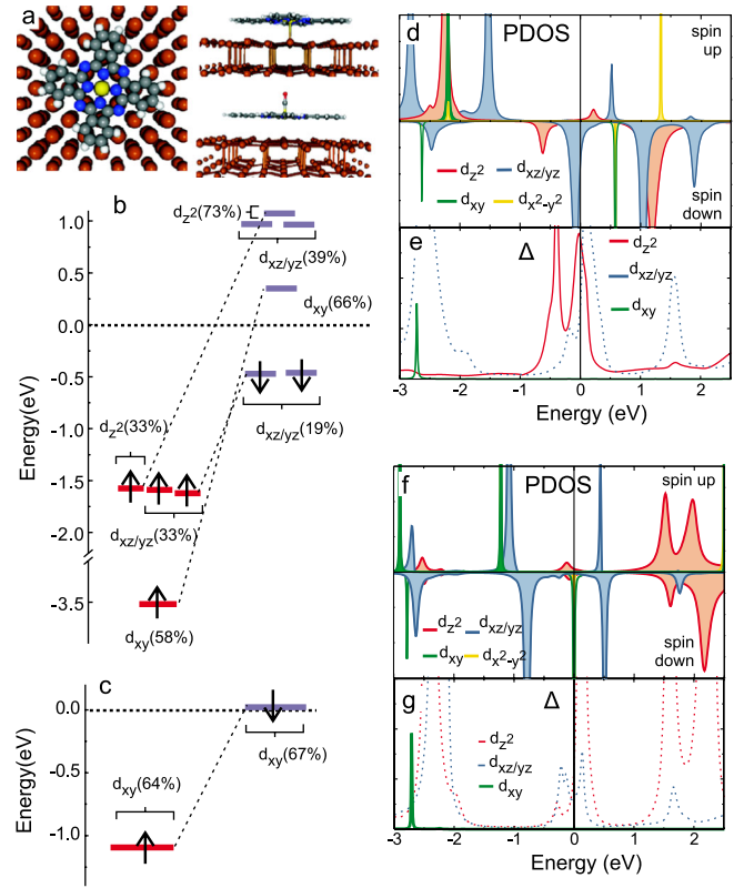
FIG. 4 (color online). (a) Model of computed system: top view (left) and side view (right) of CO-MnPc (top) and MnPc (bottom). (b), (c) Energy spectrum of adsorbed MnPc (b) and CO-MnPc (c), showing the relevant spin states. Bars in left (right) show the up (down) eigenvalues. The rate in parentheses gives the atomic character of the molecular orbital. (d), (f) Local density of states (PDOS) and (e), (g) hybridization function ( \Delta ) projected on d orbitals of adsorbed MnPc (d), (e) and CO-MnPc (f), (g). The dotted lines in (e) and (g) refer to the orbitals which are not relevant for the magnetism of the molecule.
