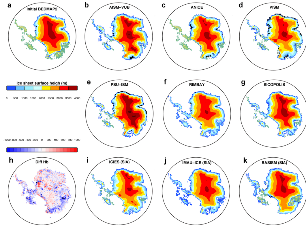
Figure 11. Ice surface topography and ice thickness of the ice shelves for the Pliocene Ice -PRISM 3 simulation with Bedmap2. (a) The initial PRISM 3 ice sheet topography modified for Bedmap2 (see text for details). (b) AISM, (c) ANICE, (d) PISM, (e) PSU-ISM, (f) RIMBAY, (g) SICOPOLIS. (h) Difference between Bedmap2 and Bedmap1 bedrock topography for the PRISM 3 initial ice sheet. SIA-only models; (i) ICIES, (j) IMAU-ICE, (k) BASISM.
