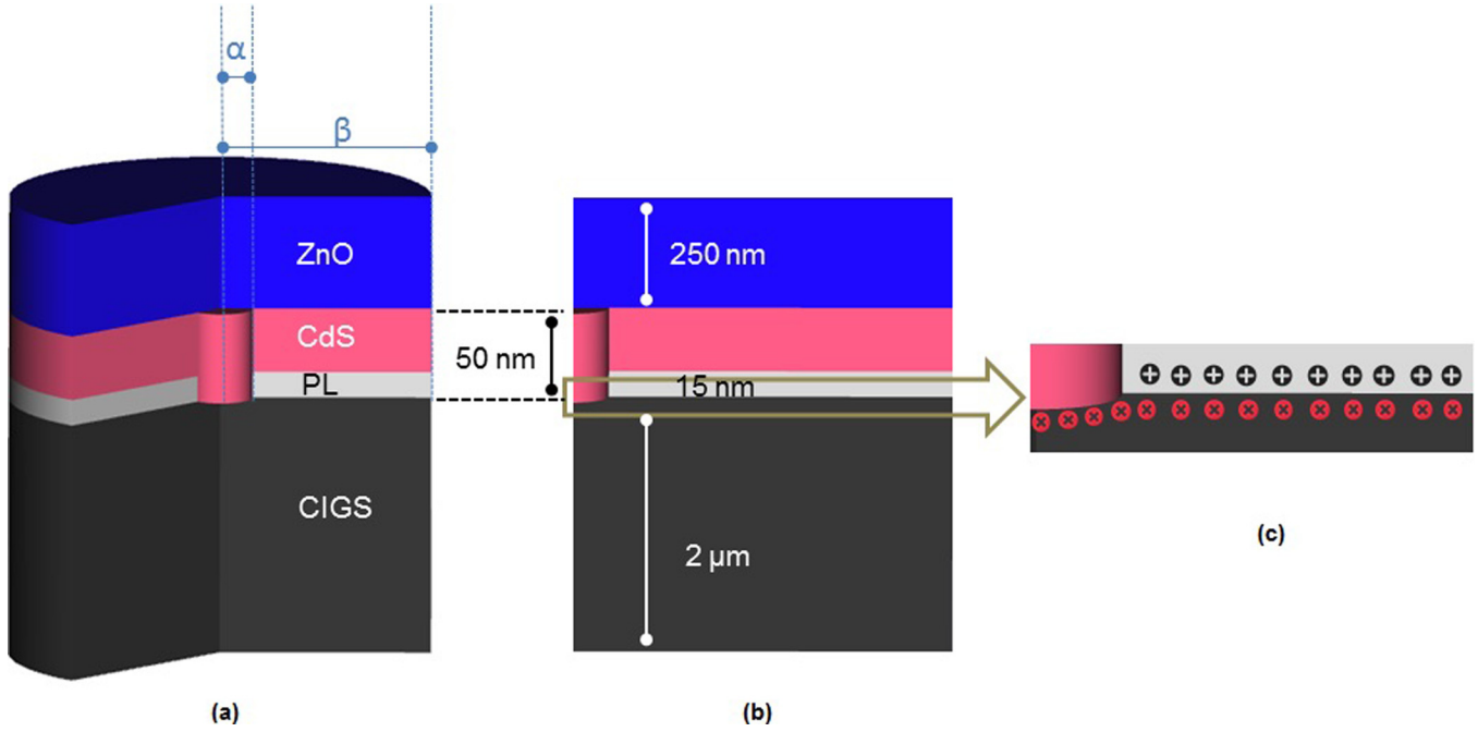
FIG. 1. Three dimensional sketch of a point-contact CIGS solar cell. \alpha : contact radius, variable, \beta : cell radius, constant at 500 nm. (a) Three dimensional overview; (b) cylindrical cut; (c) defect structure at the CIGS front interface.
