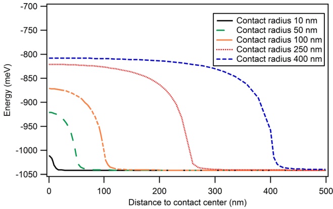
FIG. 4. Distance from valence band to Fermi-level 2 nm below the CIGS front interface. \alpha \in [10, 400] . PL defect structure, interface recombination velocity, and CBO at CIGSe/CdS similar to Fig. 2.
