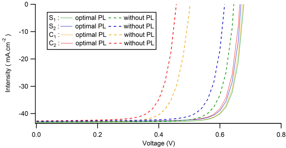
FIG. 7. J-V curves for unpassivated solar cells (dotted lines), and for passivated solar cells (solid lines). \alpha = 50\text{nm} and PL includes N_s = 2 \times 10^{14}/\text{cm}^2 density of donor trap energetically close to CIGS conduction band.
