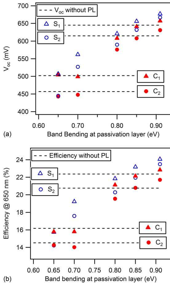
FIG. 8. Influence of \phi_{PL} on V_{oc} and efficiency. V_{oc,0} and \eta_0 (dotted lines) for unpassivated device performance. High (circles) and low (triangles) recombination velocity, 0.1 eV spike (blue empty shapes), and 0.1 eV cliff (red full shapes) at the CIGSe/CdS interface are displayed. \alpha = 100\text{nm} , so \Pi is 96%.
