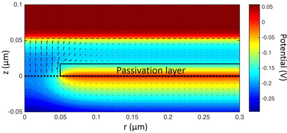
FIG. 3. Potential (color scale) and electron current (arrows) for \alpha = 50 nm. z = 0 \mu\text{m} corresponds to the CIGS front interface.
