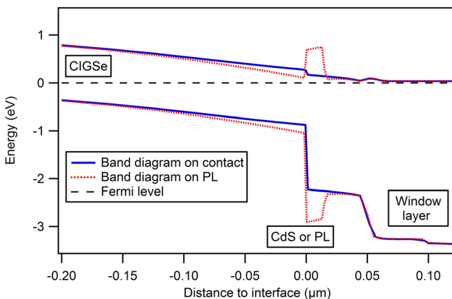
FIG. 2. Band diagram for a point-contacted solar cell. Cross-section along the z -axis close to the interface at the contact (blue curve) and on the passivation layer (red curve). \alpha = 250 \text{ nm} , and PL includes N_s^D = 2 \times 10^{14} / \text{cm}^2 density of donor traps energetically close to the CIGS conduction band. The simulated cell includes a 0.1 eV cliff at CIGSe/CdS and S = S_{max} = 2 \times 10^5 \text{ cm/s} .
