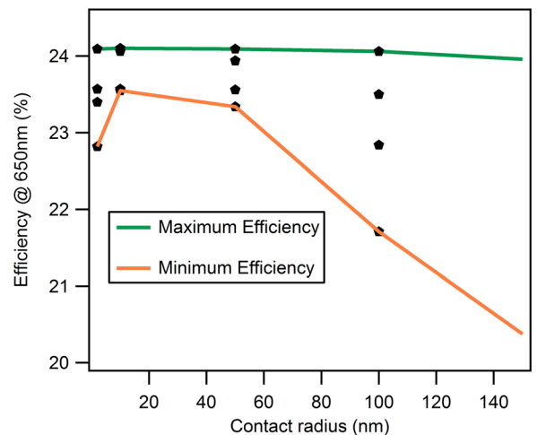
FIG. 6. Minimum and maximum efficiency for different values of \alpha . The same set of parameters as in Fig. 5.
